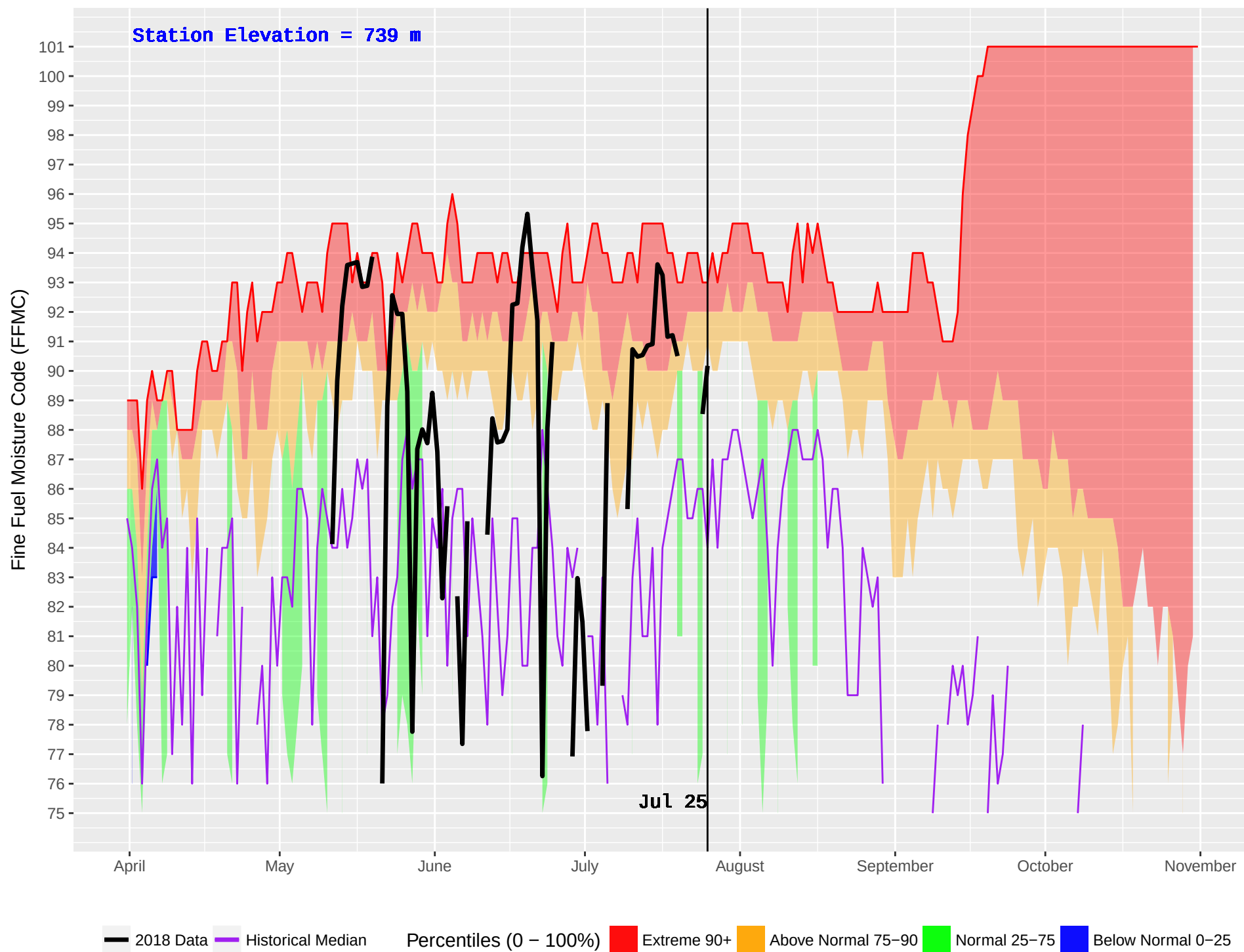
BEAR LAKE (149) : Historical (1980–2016) and Current (2018) Noon Fine Fuel Moisture Code (FFMC)
